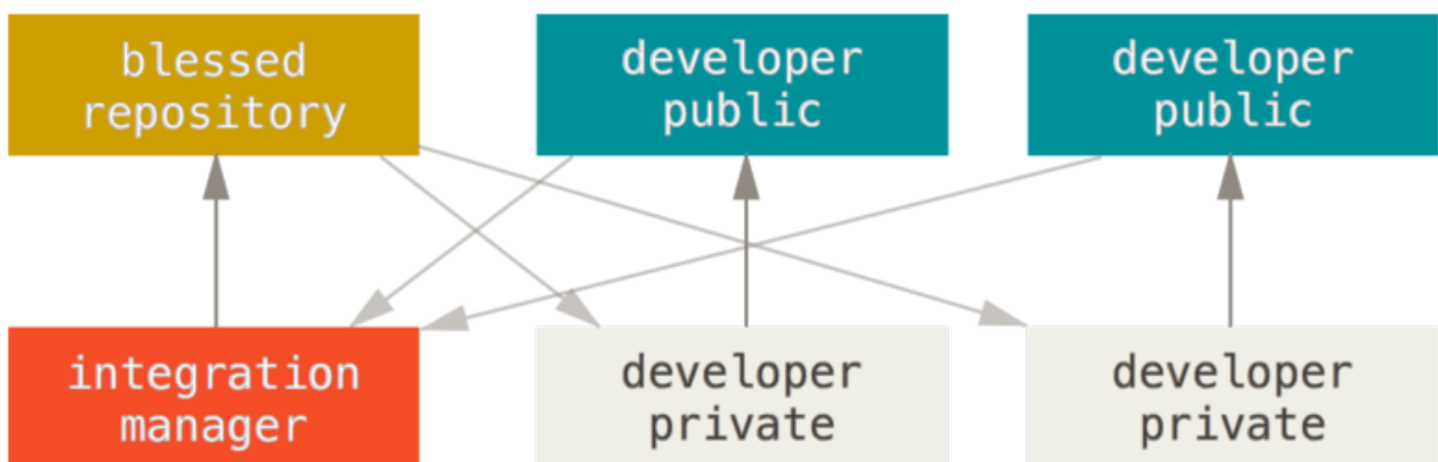
Figure 55. Integration-manager workflow.
